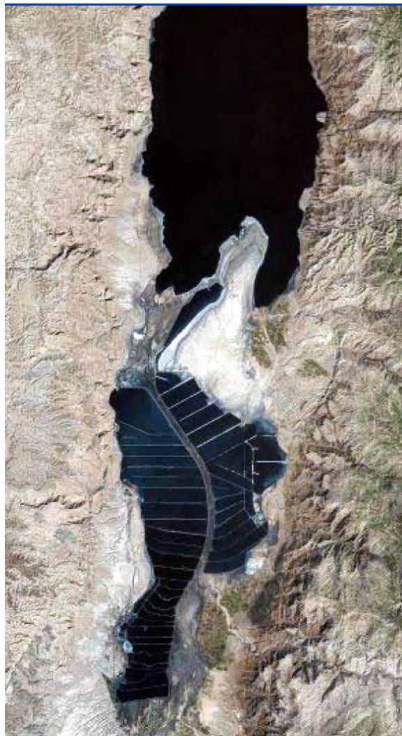
Figure 3. Enhanced satellite picture of the southern edge of the Dead Sea showing the north and south basins and the potash extraction works evaporation ponds in the southern basin. Israel's Dead Sea Works and Jordan's Arab Potash companies mine Dead Sea
